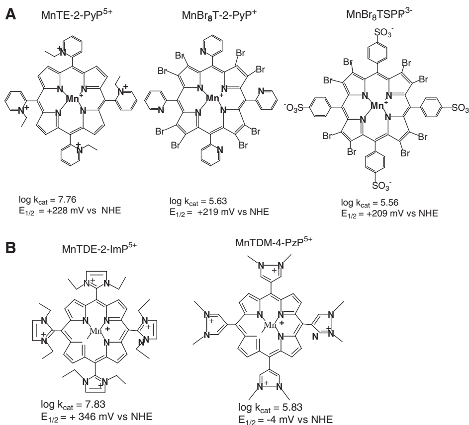
FIG. 5. The effect of charges on k_{\text{cat}} ( \text{O}_2^{\cdot-} ). Mono- vs. pentacationic porphyrins differ in k_{\text{cat}} for 2 log units, whereas cationic vs. anionic porphyrins differ in k_{\text{cat}} for more than two orders of magnitude (A), like imidazolium vs. pyrazolium porphyrins (B).
